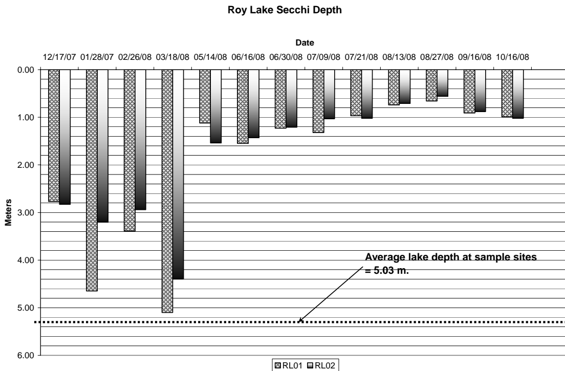
Figure 7. Secchi Depths
